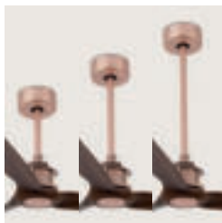
3 downrods incl. 3.9" / 7.8" / 17.7" 3 tijas incl. 100mm / 200mm / 450mm
